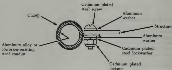
B. Bonding conduit to structure.
